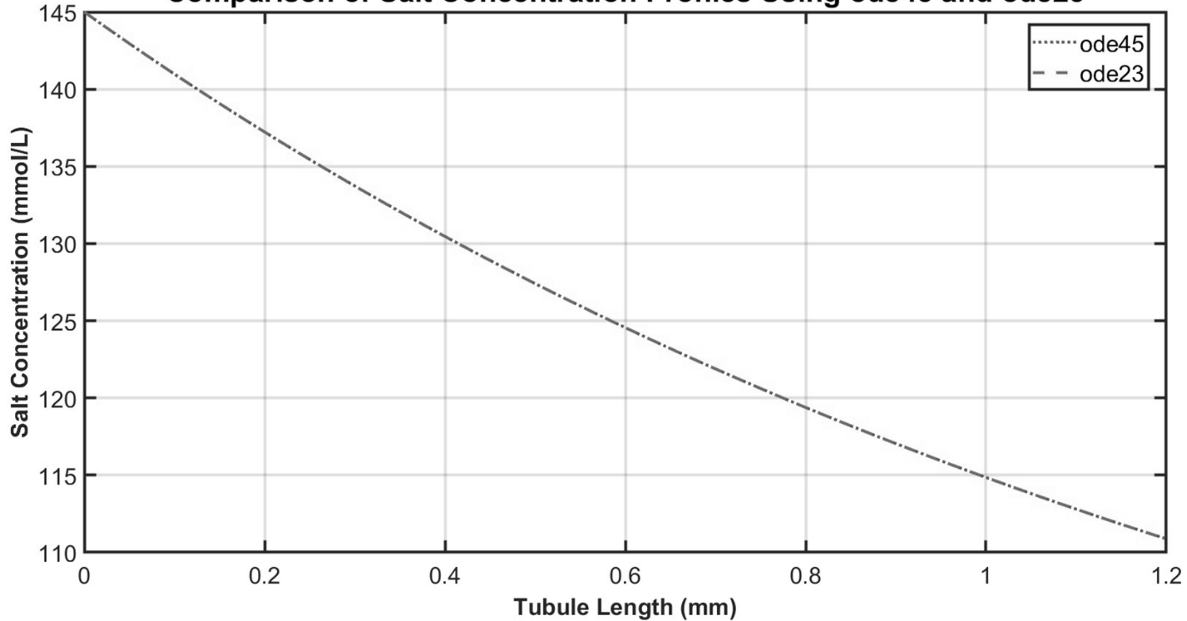
Comparison of Salt Concentration Profiles Using ode45 and ode23
